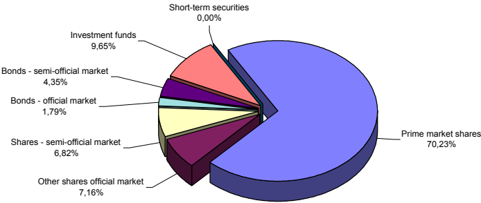
Structure of turnover by securities in May 2006
